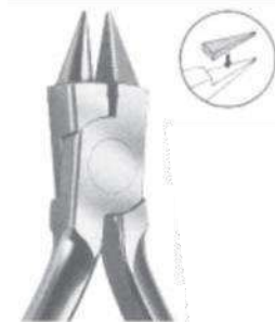
61-4071-000 Adams Plier Maximum Bending Capacity Wires up to .028" (0.7mm)
